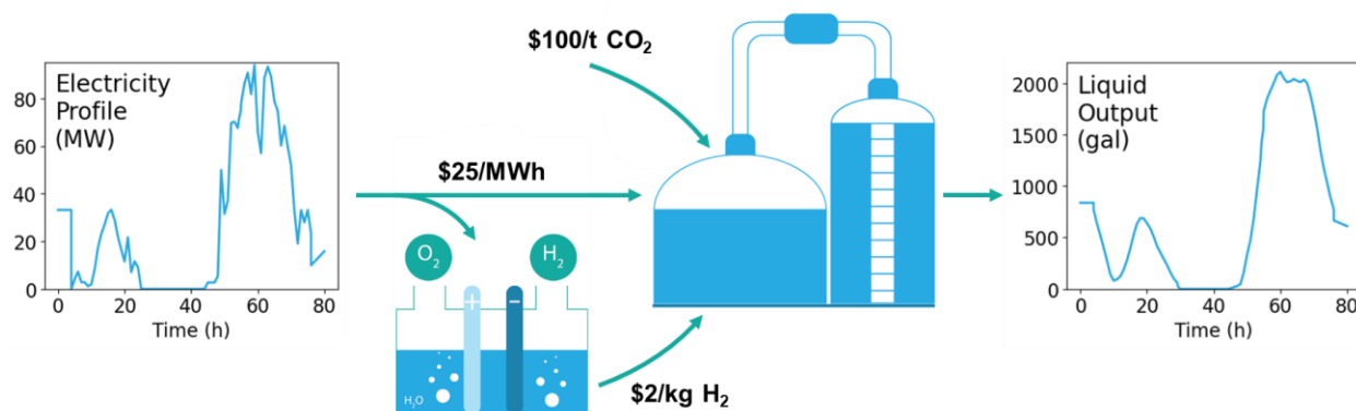
Figure 1. Black box diagram of system inputs and outputs for the reactor systems in GREENWELLS. Based on data from the Iowa State University’s Automated Surface Observing System (ASOS). 7
