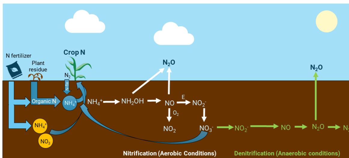
Figure 2. The N cycle for agriculture, which includes natural and anthropogenic inputs of fixed-N. The production of \text{N}_2\text{O} occurs during nitrification of \text{NH}_4^+ and denitrification of \text{NO}_3^- .
