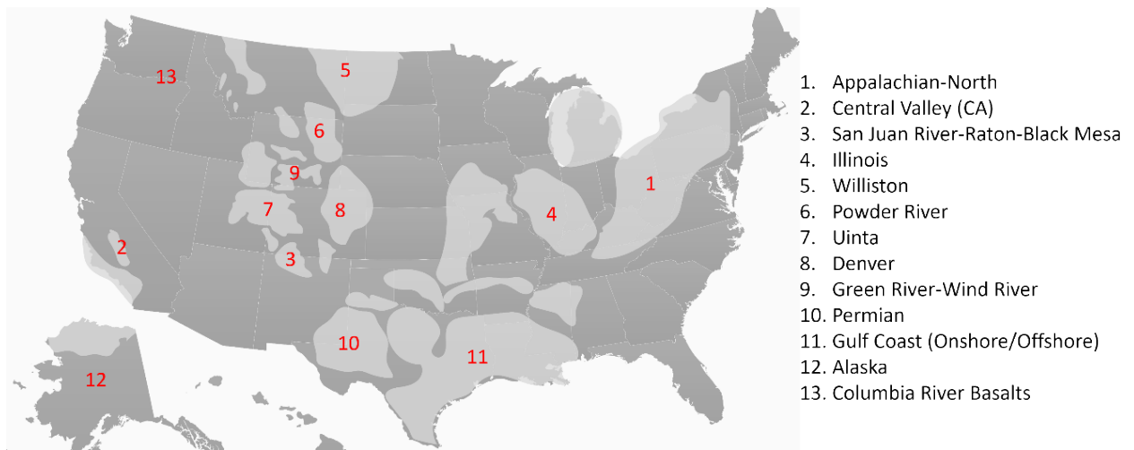
Figure 1 - Geologic Basins of the U.S.
